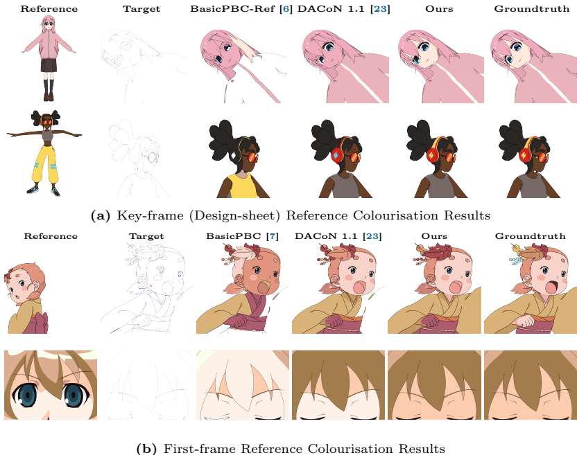
Fig. 5: Qualitative comparison under two production formulations. We show one-shot reference and target line sketch, followed by results from BasicPBC(-Ref) [6, 7], DACoN 1.1 [23], our PeCA on DACoN 1.1, and colour ground-truth (right).
